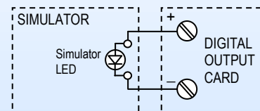
SIMULATOR SOURCING POWER FROM DO CARD
