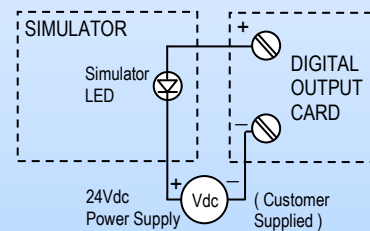
SIMULATOR EXTERNALLY POWERED
